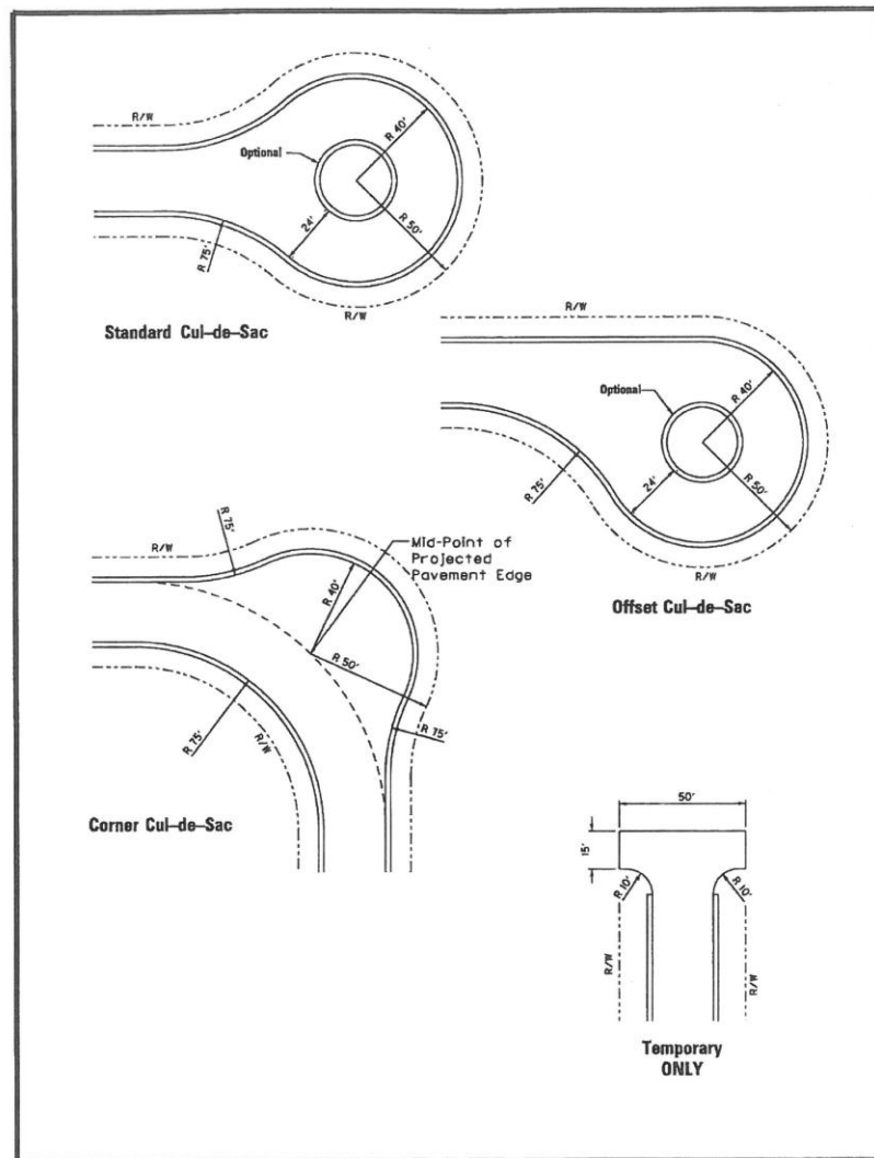
Exhibit 6-4 - CUL-DE-SACS
